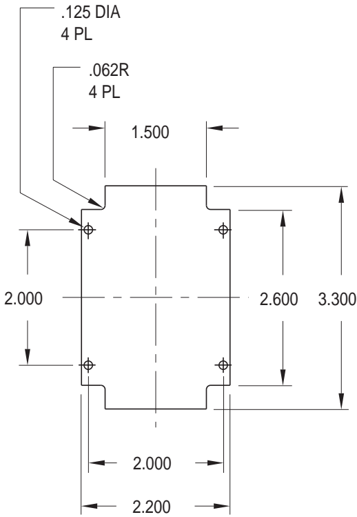
CIRCUIT BOARD REFERENCE DIMENSIONS
